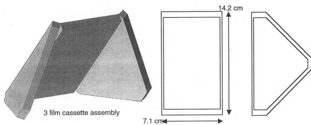
FIG. 3. Geometry for the large-angle film detector. This consists of three film holders positioned to record x rays diffracted at a wide range of angles.
