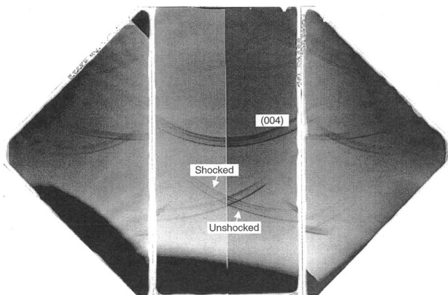
FIG. 9. Example image of x rays diffracted from shocked single-crystal Si. X rays were diffracted from both the shocked and unshocked lattice during the experiment.
