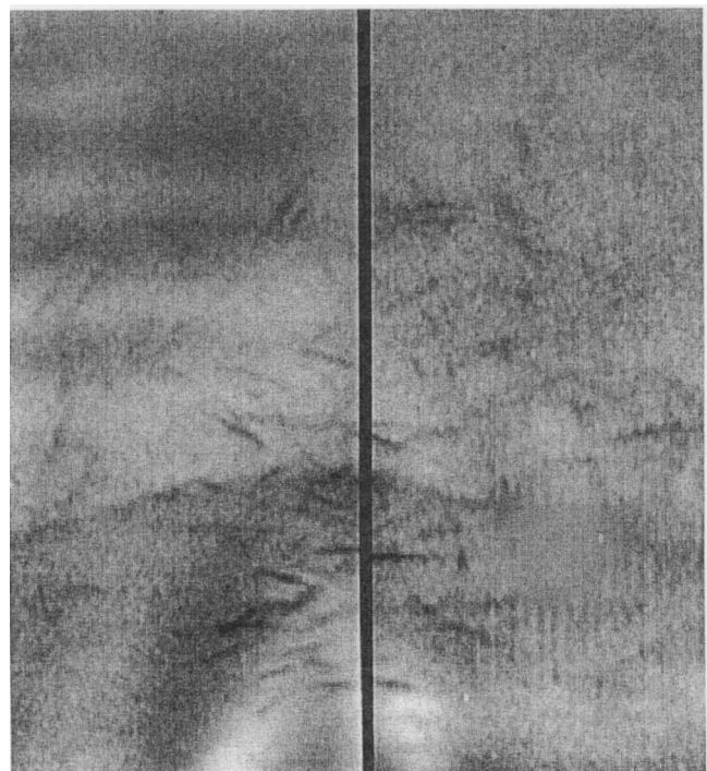
FIG. 11. Example of x rays diffracted from a polycrystal sample of Be. The presence of short diffraction lines indicates that the foil is solid and has many grains.
