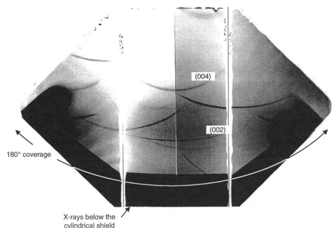
FIG. 5. Example of film data showing x rays diffracted from multiple lattice planes of single-crystal Cu. The (002) and (004) planes parallel to the surface are indicated.
