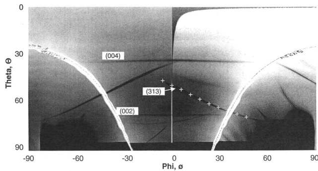
FIG. 8. Warped image of the x rays diffracted from single-crystal Cu displayed in angle space. The data cover an angular range of 90° in the vertical direction and 180° in the horizontal direction.
