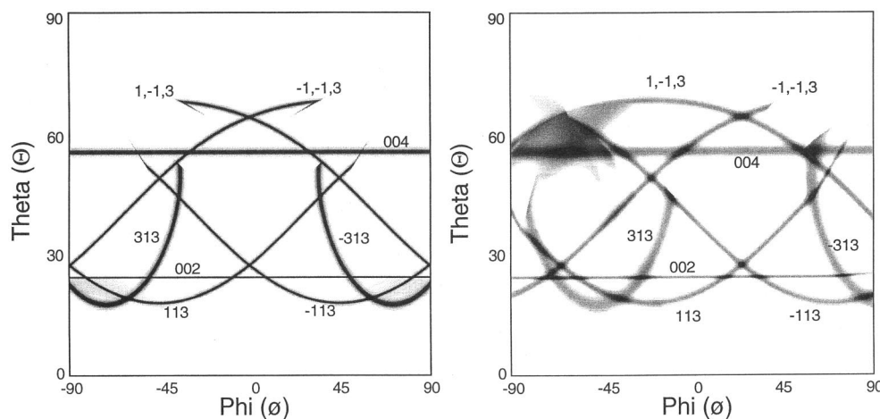
FIG. 7. Calculated diffraction signals for specific lattice planes of single-crystal Cu using a Cu x-ray source at 1.49 \text{ \AA} . The relative orientation of the lattice is rotated by 20^\circ for the image on the right.
