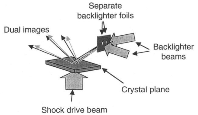
FIG. 10. Geometry for in situ diffraction using two separate backlighter foils to provide dual images with time resolution.
