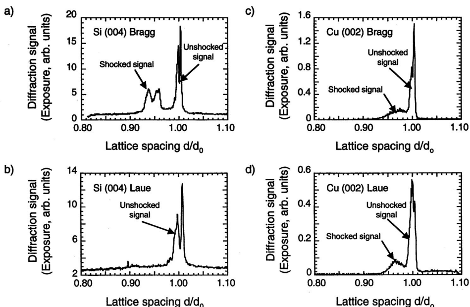
FIG. 2. Lineouts showing the compression of single-crystal Si and Cu. For single-crystal Si, there is compression of the lattice parallel to the shock direction (a), but not perpendicular (b). For single-crystal Cu, there is compression of the lattice both parallel (c) and perpendicular (d) to the shock direction. Note that the unshocked feature has structure due to the spectrum of the x-ray source.
