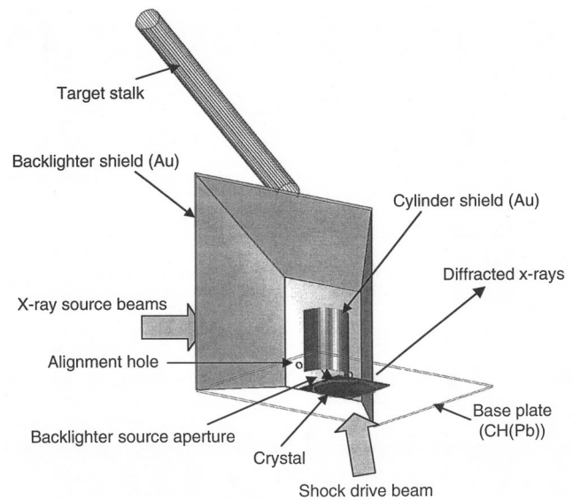
FIG. 4. Example of the target used for the in situ shock compression experiments. This is approximately 8 mm in size.
