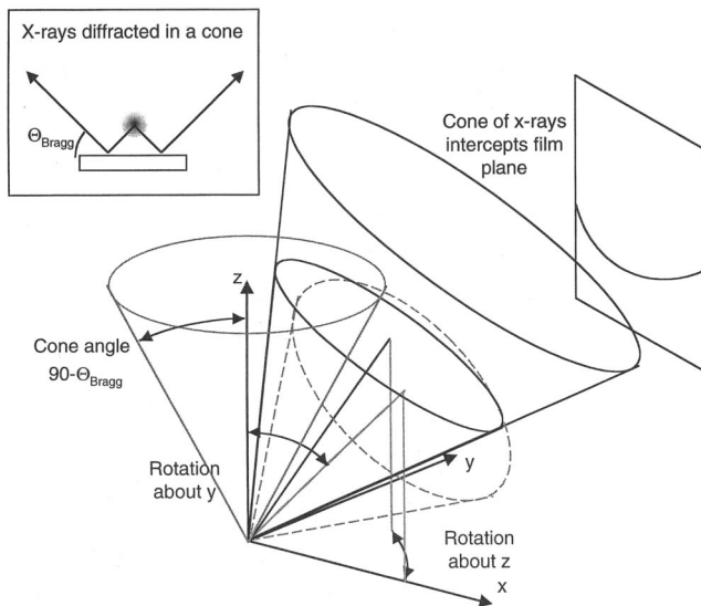
FIG. 6. Geometry that is used in the fit routines for the diffraction signals. Each arc on the film is due to a cone of x rays diffracted from a specific lattice plane in the crystal. The best fit cone for each line is given by three angle parameters that represent the Bragg angle and lattice normal vector.
