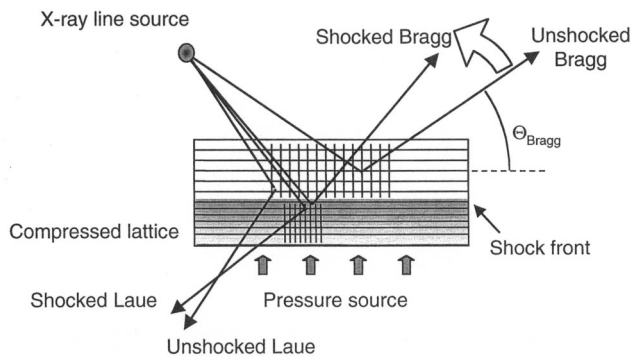
FIG. 1. Schematic showing the geometry for in situ x-ray diffraction. Compression of the lattice spacing is observed as a shift in the Bragg angle of the diffracted x rays.
